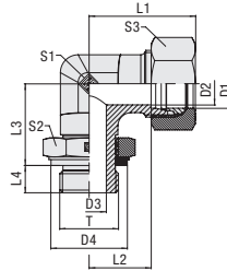
Whitworth Parallel Pipe Thread (BSP)
