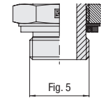
O-Ring with Retaining Ring (Adjustable)
