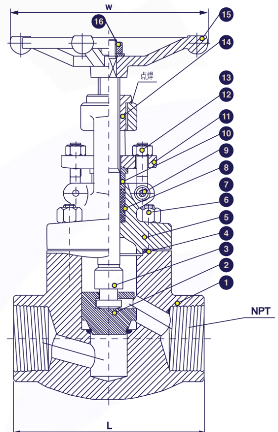
Threaded End SS316 Globe Valves 800 PSI
